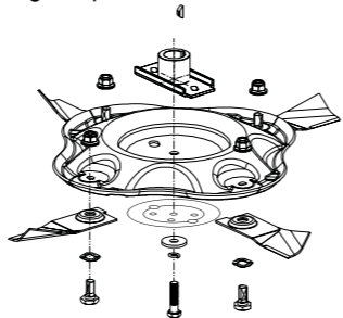
Lama Quadcut®
