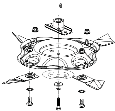
Cuchilla "Quadcut"
