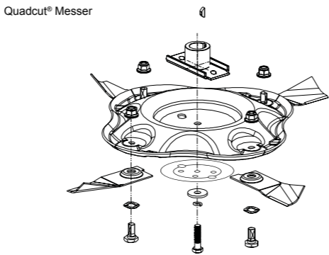
Quadcut® Messer
